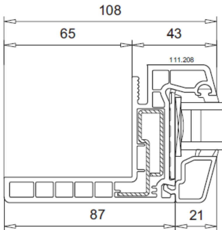
111.208 varianta 0
