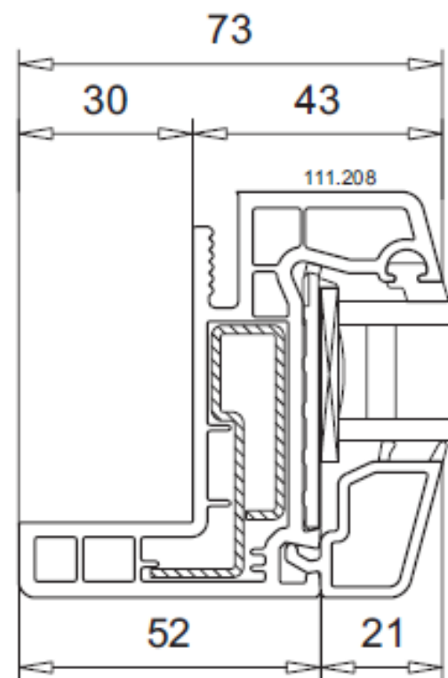
111.208 varianta 1
